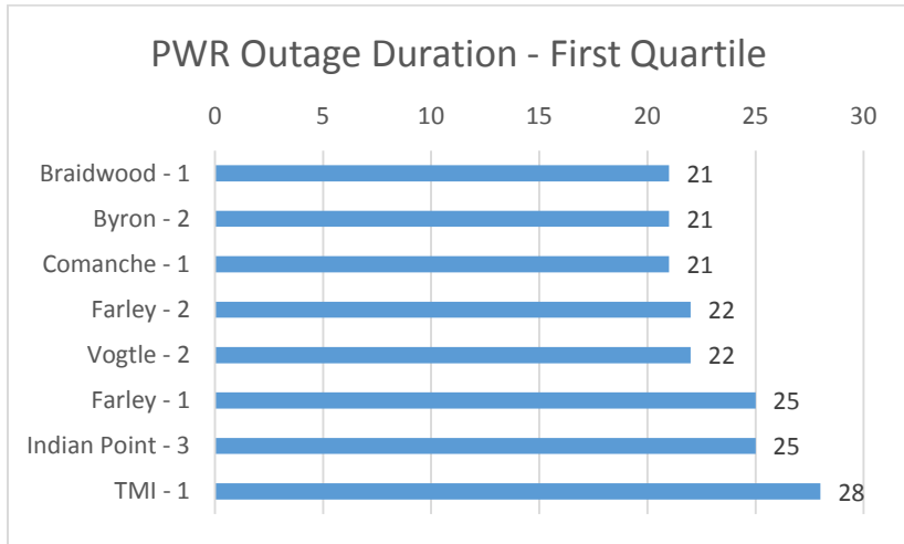
Figure 1. 2013 PWR Outage Duration Quartiles
