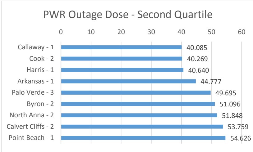
Figure 2. 2013 PWR Outage Dose Quartiles
